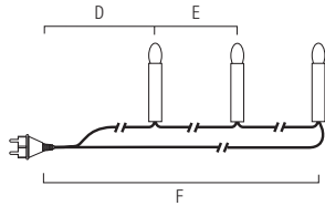
Christmas tree lights without split plug
