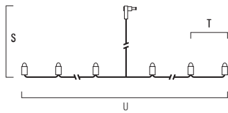
Parallel connected/double insulated light set
