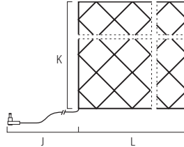
Net light set
