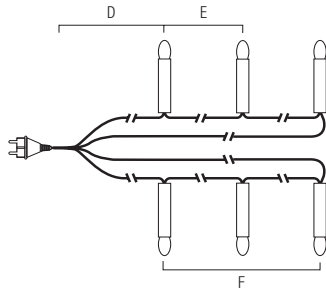
Christmas tree lights without split plug
